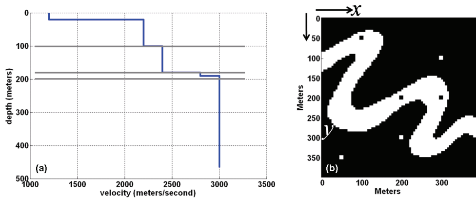
Figure1: (a) The velocity variation (blue lines) and reflectors (grey lines) for the exhaustive model. (b) The reflectivity function for the reflector at 200m depth. Black indicates a value of +0.1 and white is -0.1.
