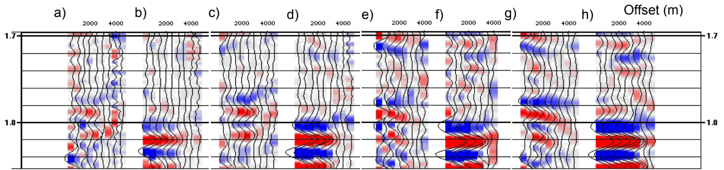
Figure 3: Ostrander gather at well A (a) & B (b), interpolated Ostrander gather at well A (c) & B (d), PSTM Ostrander gather at well A (e) & B (f), interpolated PSTM Ostrander gather at well A (g) & B (h). The Viking is at 1790 ms at well A and 1821 ms at well B.
