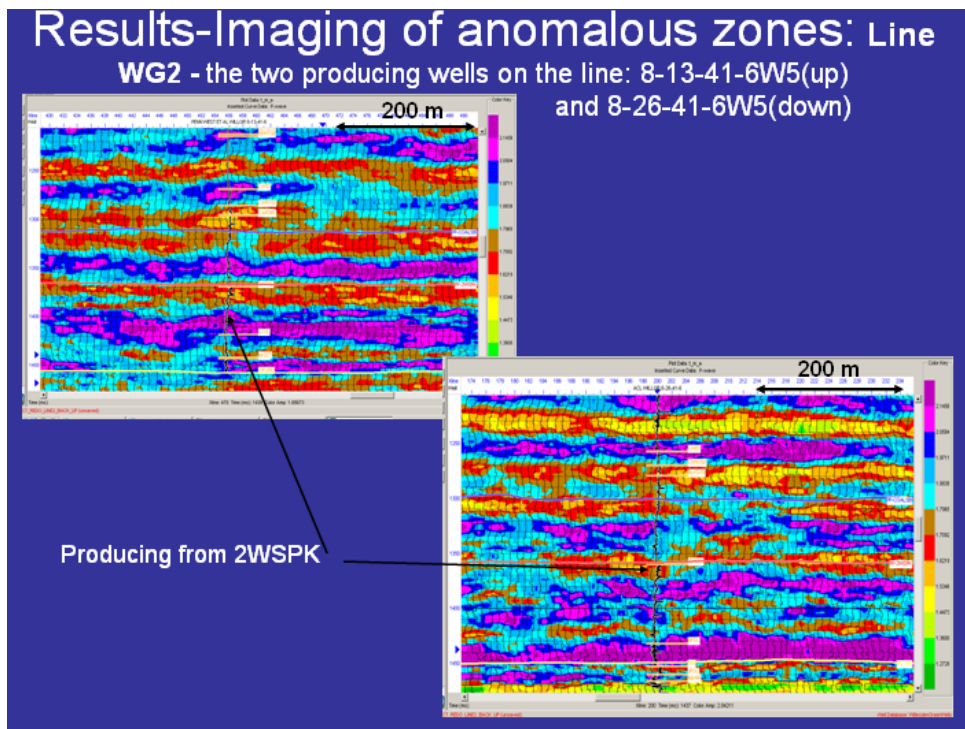
Figure 4. Delineation of anomalous zones: the ratio of the PP inversion to PS inversion in PP time on line WG2 at the two producing wells 8-13-41-6W5 and 8-26-41-6W5.
