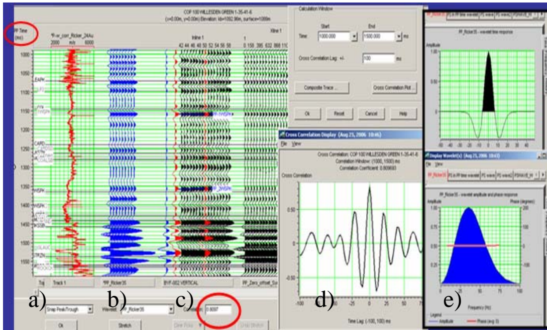
Figure 3. Synthetic, seismic and well log correlation at well 1-35-41-6W5:
