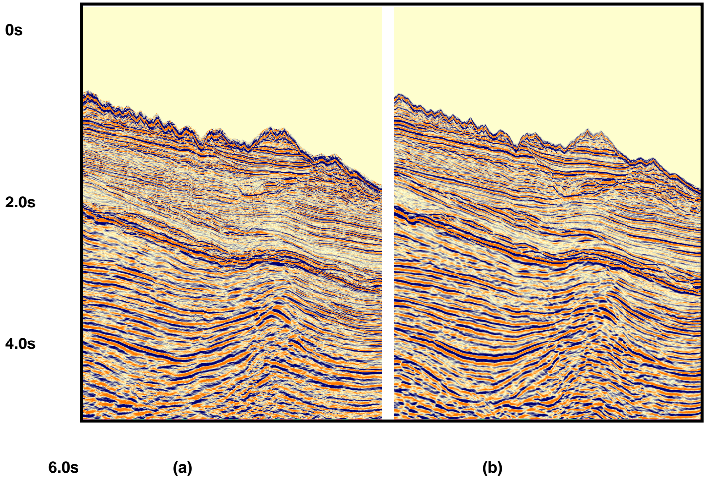
Figure 3b. An inline Stack; (a): PreSTM & (b): PreSDM converted to time.
