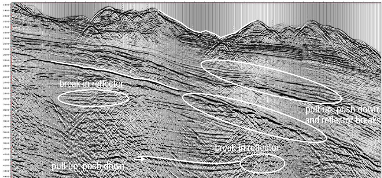
Figure 1. Original seismic inline illustrating the rugosity of the sea floor and its impact on the time image that cannot be solved by 3D PreSTM but requires 3D PreSDM
