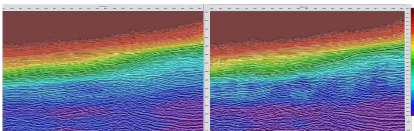
2 nd iteration PreSDM velocity model
