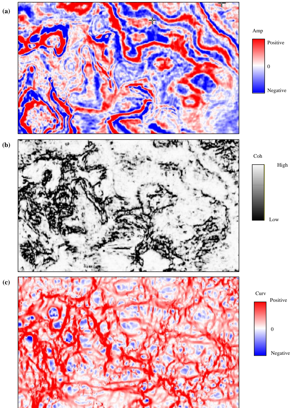
Figure 2. Time slices at 2104 ms through (a) seismic, (b) coherence, and (c) most-positive curvature volumes. Notice that while the coherence display is featureless in the high coherence (white) areas, most-positive curvature delineates N-S flexures in those areas. Also note the through-going E-W flexure in the southern part of the survey. (Data courtesy of Oilexco, Calgary).
