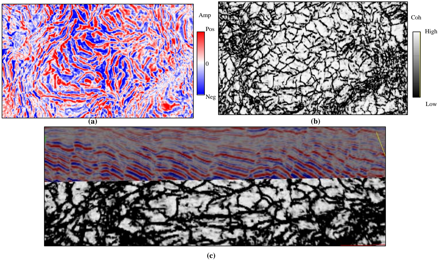
Figure 1. Time slice at 1240 ms through (a) a seismic volume from North Sea, (b) the equivalent coherence slice generated using a modified eigendecomposition algorithm with a robust dip-steering option. Notice the accurate imaging of the fault pattern seen on the coherence slice in (b), which is almost impossible to detect on the seismic. (c) shows a chair display of the fault patterns on the coherence and a vertical seismic section. This helps correlate the fault breaks with their seismic signatures. (Data courtesy of Oilexco, Calgary)
