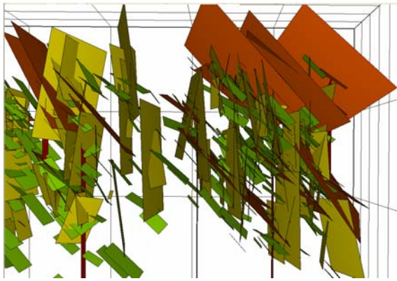
Figure 4 Detail of Discrete Fracture Network (DFN) model based on hierarchical model following Flodin (2003).
