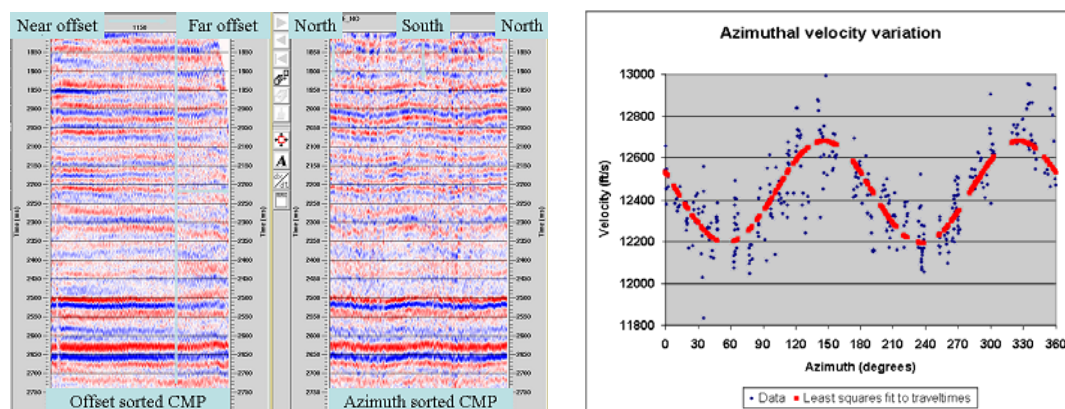
Figure 1. Offset and azimuth sorted gathers, Rocky Mountains
