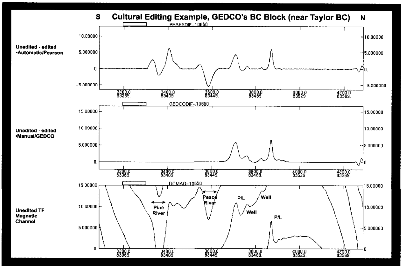
Fig. 2. Cultural editing example for a profile in same data set as Fig. 1. The vertical scale on all profiles is in nT. The upper annotation is sample number (about one sample every 6-8 m, depending on aircraft speed), and the lower annotation is fiducial (FID) number. The lower profile is the unedited magnetic field, the middle profile is the difference between the unedited data and manual edited data, and the top profile is the difference between the unedited data and semi-automatic edited data. The magnetic response of the Peace and Pine River Valleys reflects both the terrain effect of the river valleys, where iron-rich Cretaceous sediments outcrop in the valley walls, and the magnetic signature of deeper fault control, which controls the courses of both rivers.
