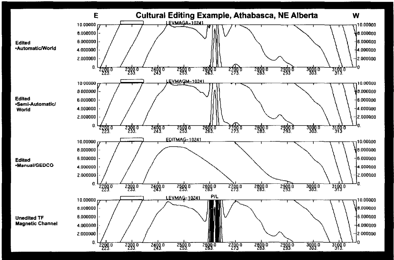
Fig. 3. Cultural editing for a profile in the Athabasca area (Best et al., 1998, this volume). The lower profile is the unedited data, the next profile is manually edited data, the next profile is the semi-automatic version of the culturally suppressed data, and the top profile is the automatic version of the culturally suppressed data.
