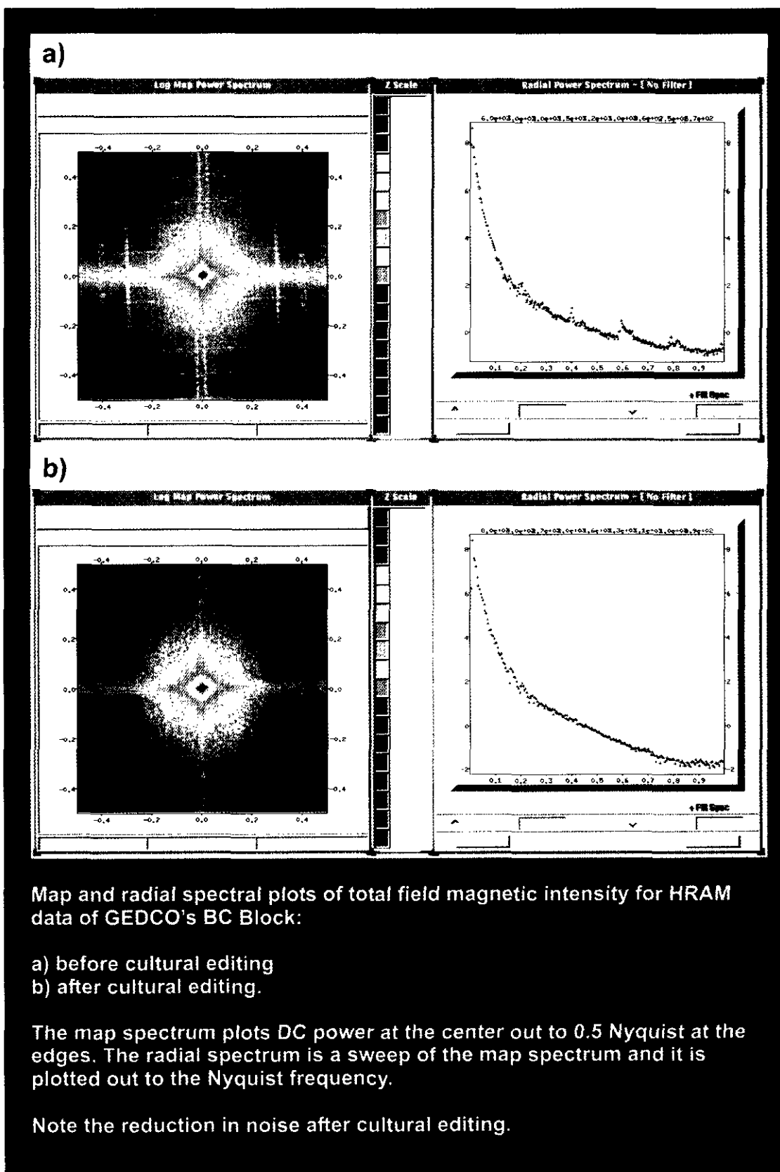
Fig. 1. Map and radial spectral plots of total magnetic field for data from the Peace River area in northeast British Columbia: a) before cultural editing; and b) after manual cultural editing. The map spectrum plots DC power at the center out to 0.5 Nyquist at the edges. The radial spectrum is a sweep of the map spectrum and is plotted out to the Nyquist frequency.
