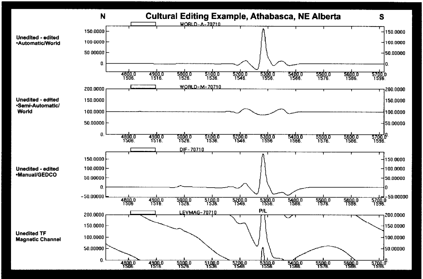
Fig. 4. Cultural editing for a profile in the Athabasca area. The lower profile is the unedited data, the next profile is the difference with manually edited data, the next profile is the difference with the semi-automatic version of the culturally suppressed edited data, and the top profile is the difference with the automatic version of the culturally suppressed data.
