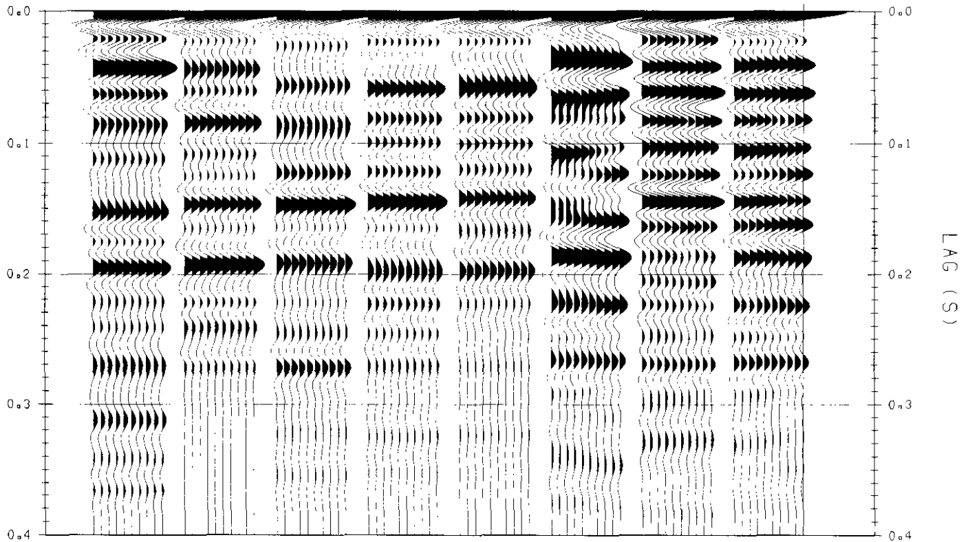
Fig. 5. Autocorrelations of assimilated data for the reef well. The calculation window ranges from 0.8 s to 1.2 s. From left to right is the interbed multiples synthetic, primary synthetic, 60 ms corridor, 200 ms corridor, full VSP corridor stack, far stack, near stack, and full stack. Prediction distance can only be chosen based on the VSP.
