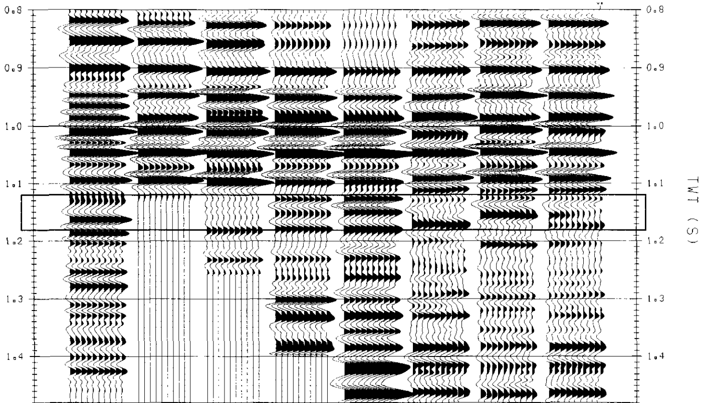
Fig. 4. Assimilation of data for the reef well. From left to right is the primaries plus all interbed multiples synthetic (impulse response neglecting surface reflector), primary synthetic (35 Hz Ricker), outside VSP corridor stack (60 ms window), outside corridor (200 ms window), full VSP corridor stack, far stack (1000-2000 m), near stack (200-1000 m), and full CDP stack (200-2057 m).
