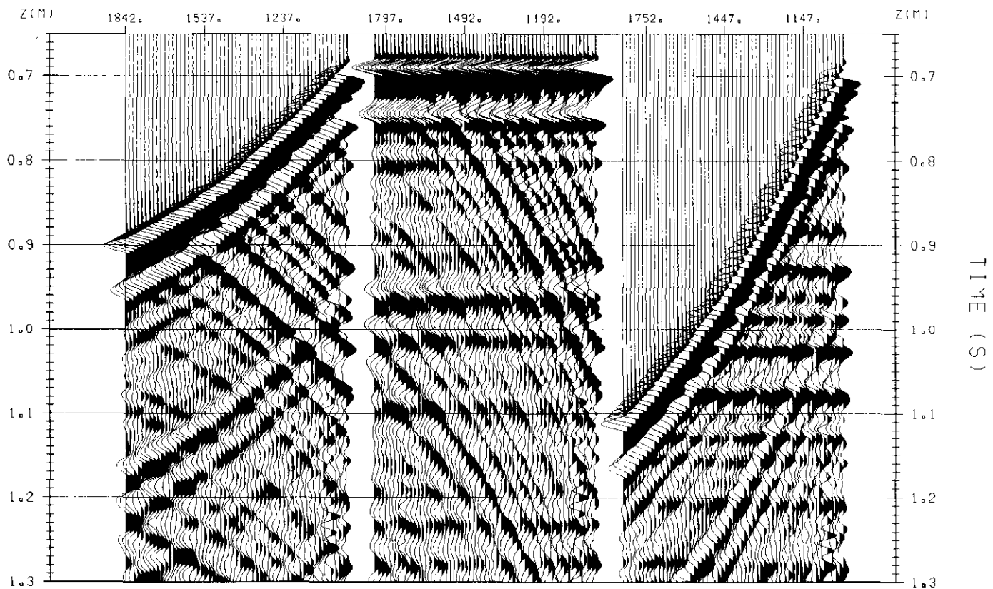
Fig. 2. Various processing time frames for the reef VSP. From left to right is field record time (FRT), first break advance time ( -TT ), and first break delay time ( +TT ). In -TT time, downgoing VSP events are delayed relative to the initial downgoing compression by the TWT between the generating interface and the deeper reflector. These events are recorded only at depths below the generating interface. In +TT time, upgoing VSP events are positioned to the TWT at which they are recorded. First breaks were optimized by correlation statics, and bulk has been applied to match surface data.
