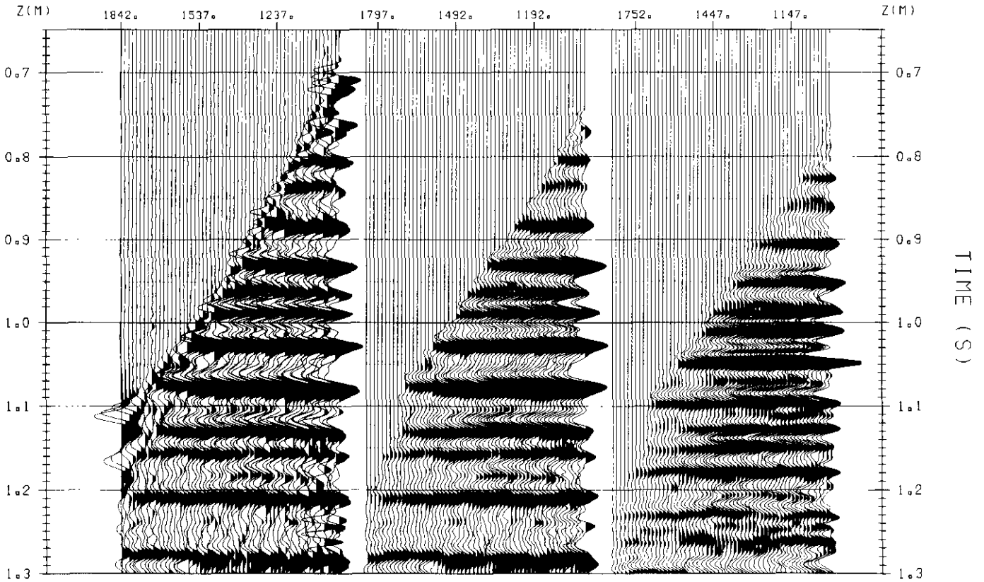
Fig. 3b. Processing stages for the upgoing wavefield (+TT). From left to right is the f-k separated wavefield, output from trim statics and median filtering, and finally waveshaped using the downgoing compressional wavefield. The outside corridor stack can be produced by muting all data below a delayed first break trajectory before stacking. Note that residual f-k energy was muted near the edges of the record.
