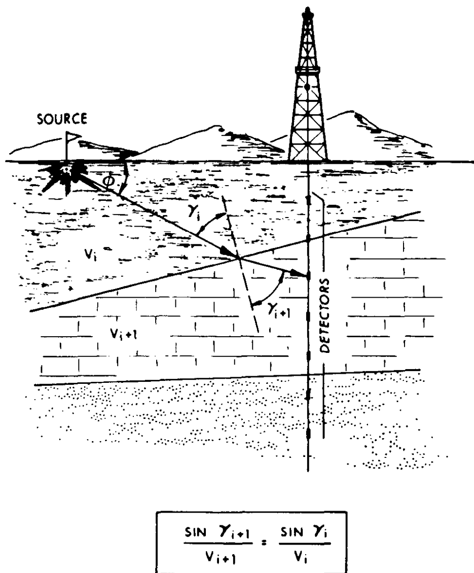
Fig. 1. Vertical seismic profiling recording configuration – from Lines et al. (1984).
