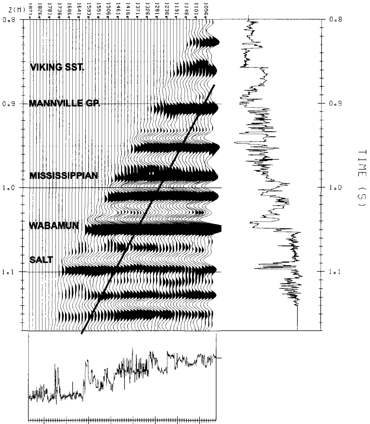
Fig. 3c. Wavelined upgoing VSP wavefield (+TT) compared to impedance logs in time (constrained by corrected checkshots) and in depth (TVD, SRD = 900 m). The concept of inside corridor stacking is illustrated by the mute zone. Some geologic entities are identified.
