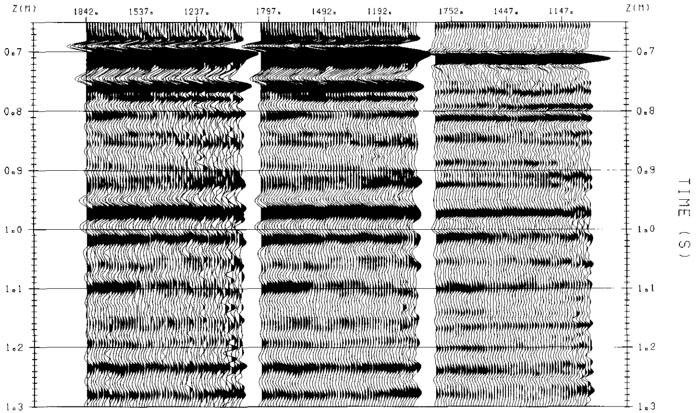
Fig. 3a. Processing stages for the downgoing wavefield (-TT). From left to right is the f-k separated wavefield, output from median filtering, and finally waveshaped using the average wavelet contained within an 80 ms window starting at the first peak.
