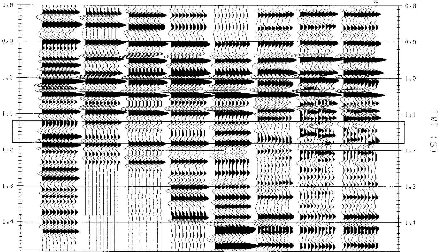
Fig. 6. Assimilation of data for the reef well following predictive decon using 60 ms operator length and 90 ms prediction distance. From left to right is the impulse response synthetic, primary synthetic, 60 ms corridor, 200 ms corridor, full VSP corridor stack, far stack, near stack, and full stack.
