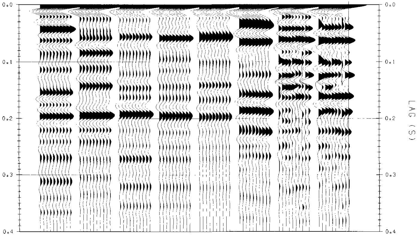
Fig. 7. Autocorrelations of assimilated data for the reef well following predictive decon using 60 ms operator length and 90 ms prediction distance. The correlation window ranges from 0.8 s to 1.2 s. From left to right is the impulse response synthetic, primary synthetic, 60 ms corridor, 200 ms corridor, full VSP corridor stack, far stack, near stack, and full stack.
