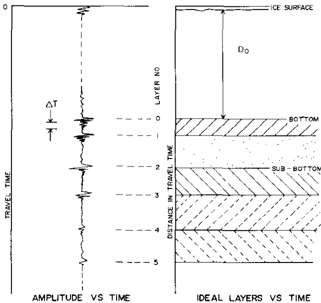
Fig. 3. Physical reflection model.
