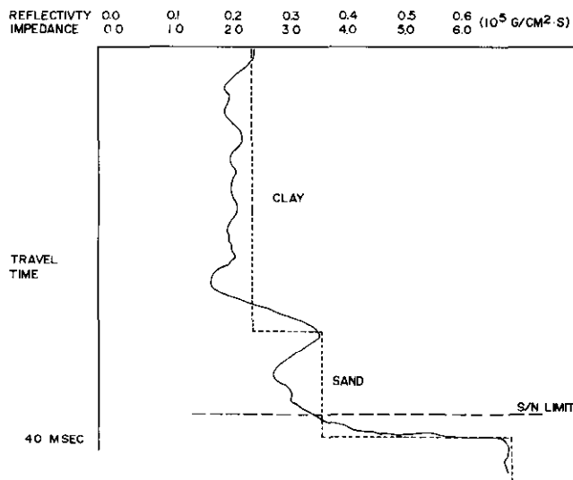
Fig. 4. Acoustic impedance as a function of travel time.
