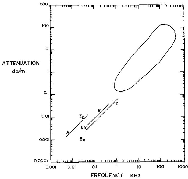
Fig. 1. Attenuation as a function of frequency (reproduction of Hamilton, 1972).
