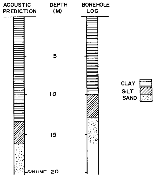
Fig. 10. Acoustic prediction versus borehole log.
