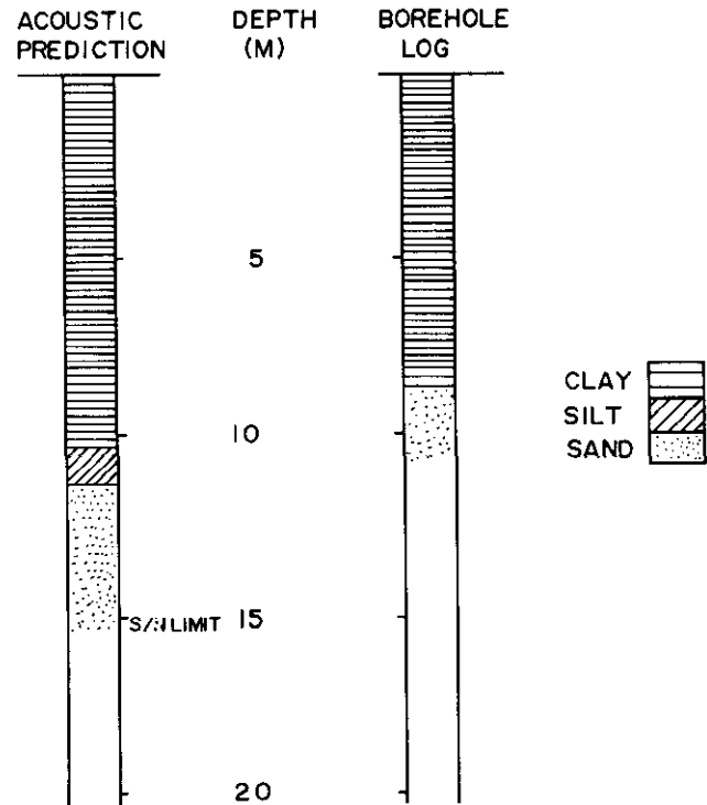
Fig. 7. Acoustic prediction versus borehole log.
