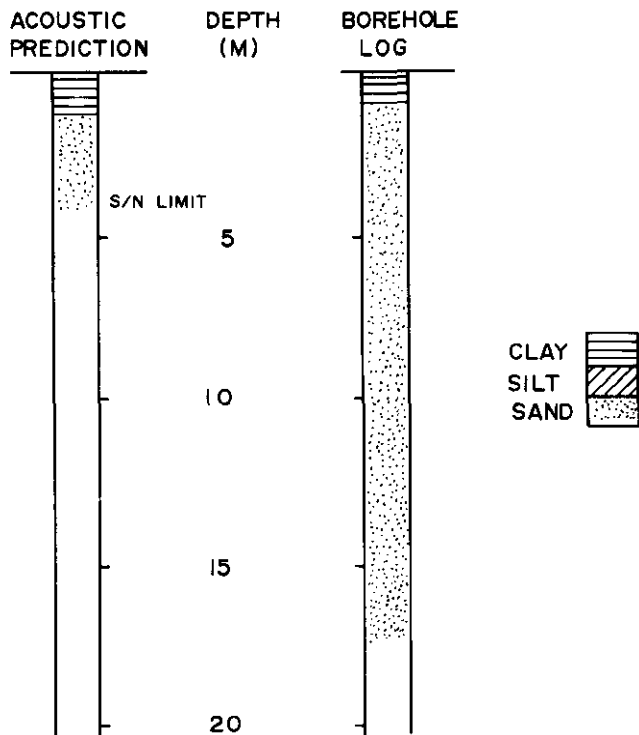
Fig. 9. Acoustic prediction versus borehole log.
