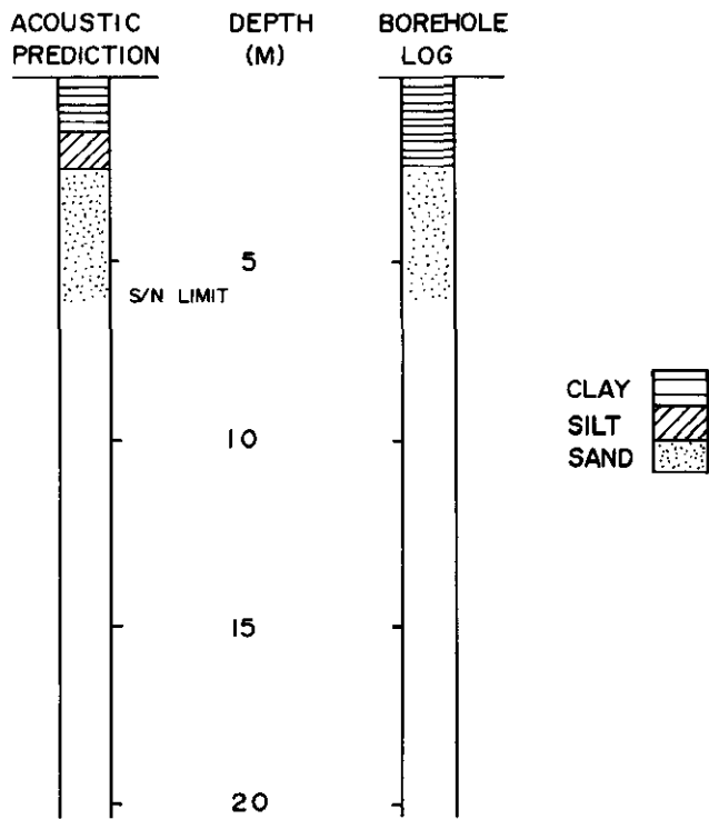
Fig. 8. Acoustic prediction versus borehole log.
