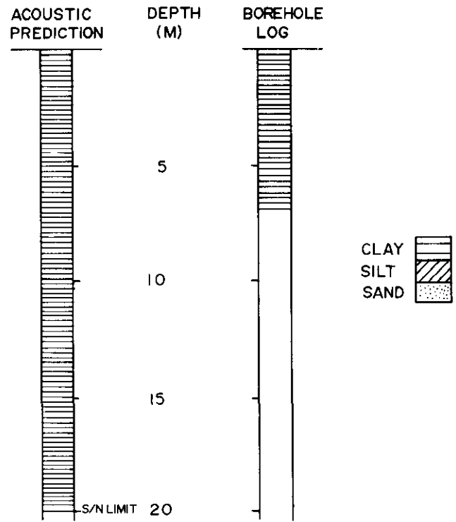
Fig. 6. Acoustic prediction versus borehole log.
