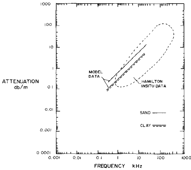
Fig. 2. Model attenuation prediction versus Hamilton (1972) in situ measurements.
