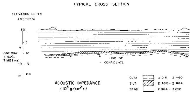
Fig. 5a. Acoustic impedance and soil classification for the sediment in the Beaufort sea.
