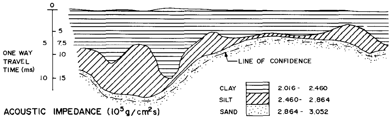
Fig. 11. Typical cross section of a river bed.
