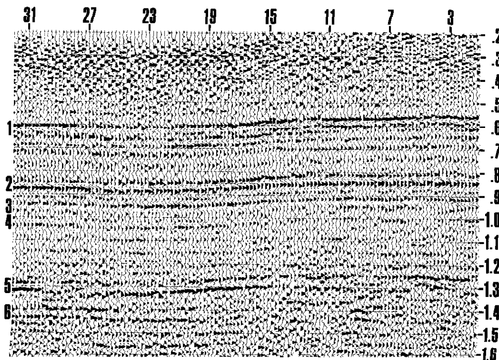
Fig. 4. A 12-fold stack section from Western Canada.
