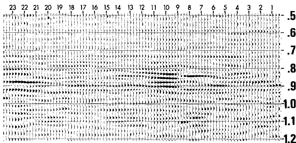
Fig. 14. The residual section computed from data in Figures 12 and 13.
