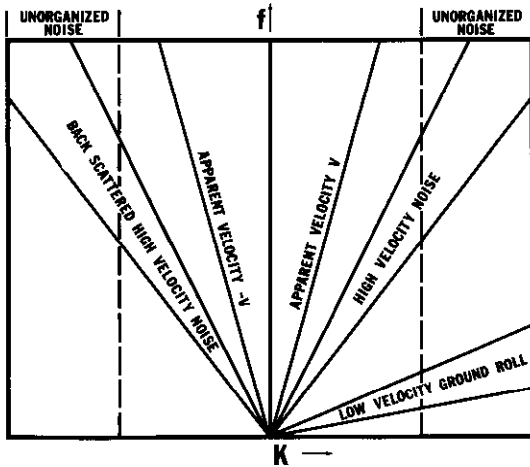
Fig. 2. Distribution of various patterns on a frequency-wave number plot (after Embree et al, 1963).
