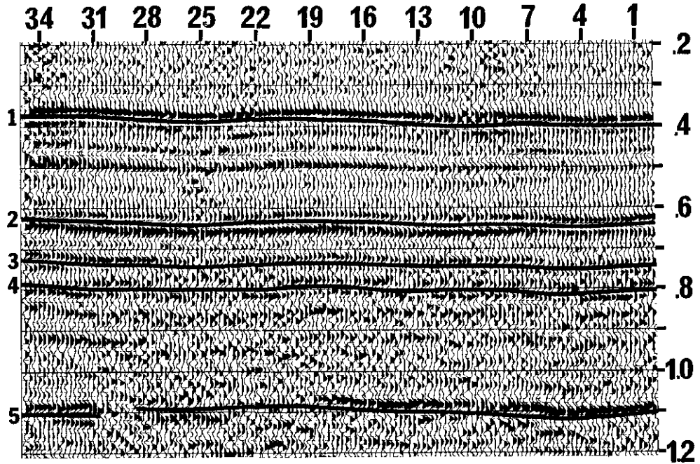
Fig. 9. Same data as in Figure 6 except that CDP gathers were processed through a two-dimensional filter before stack.
