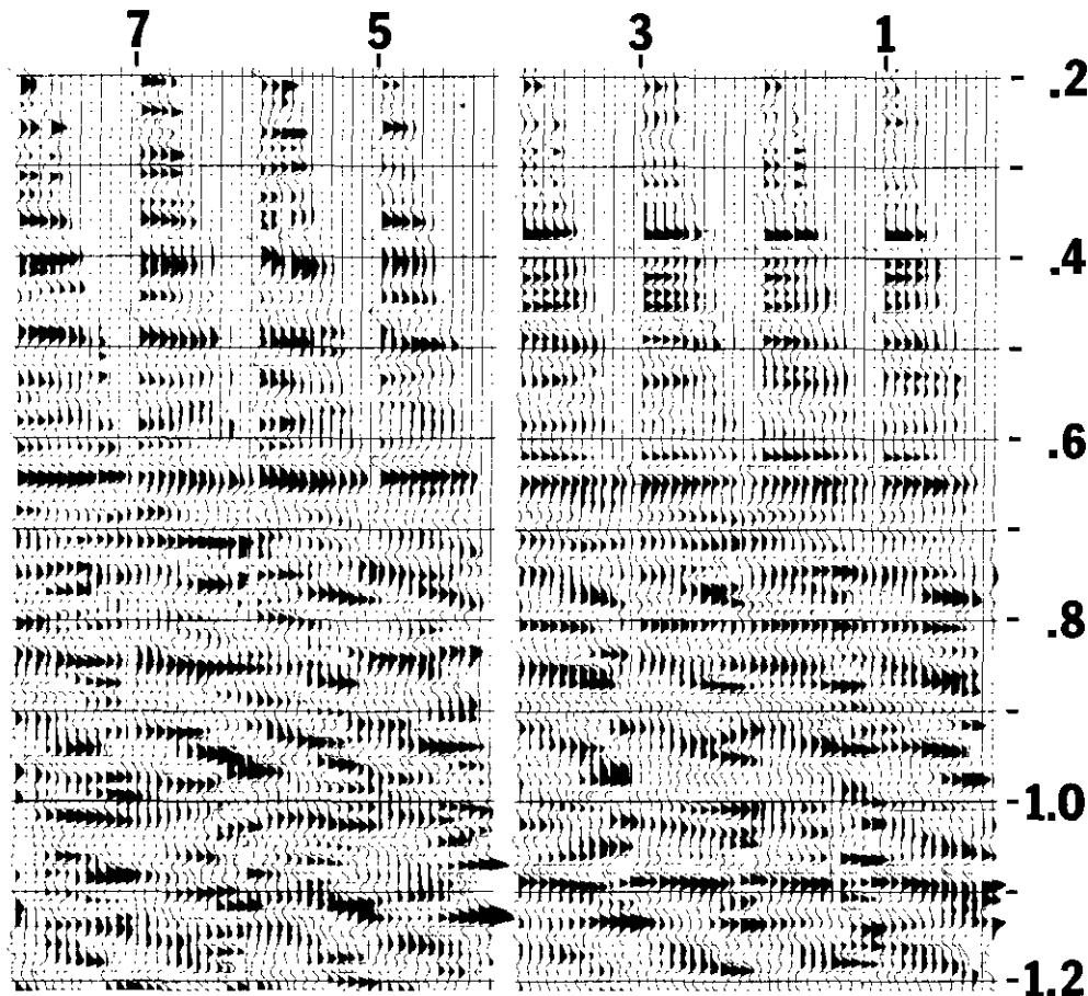
Fig. 8. Data in Figure 7 after two-dimensional filter.
