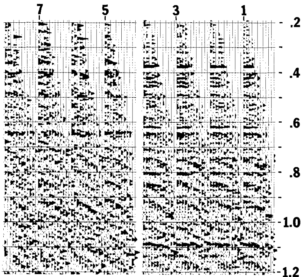
Fig. 7. An example of CDP gather of data for section in Figure 6.
