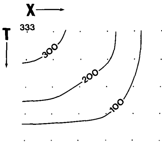
Fig. 1. Impulse response of two-dimensional filter, passband 83hz and 10 traces.
