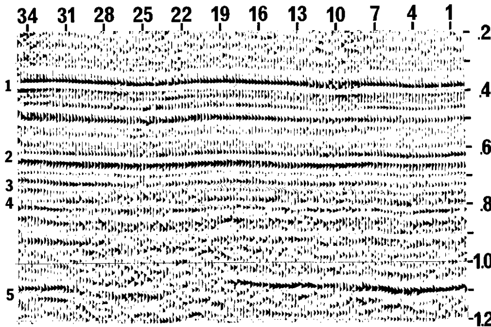
Fig. 6. A 12-fold stack section from Western Canada.
