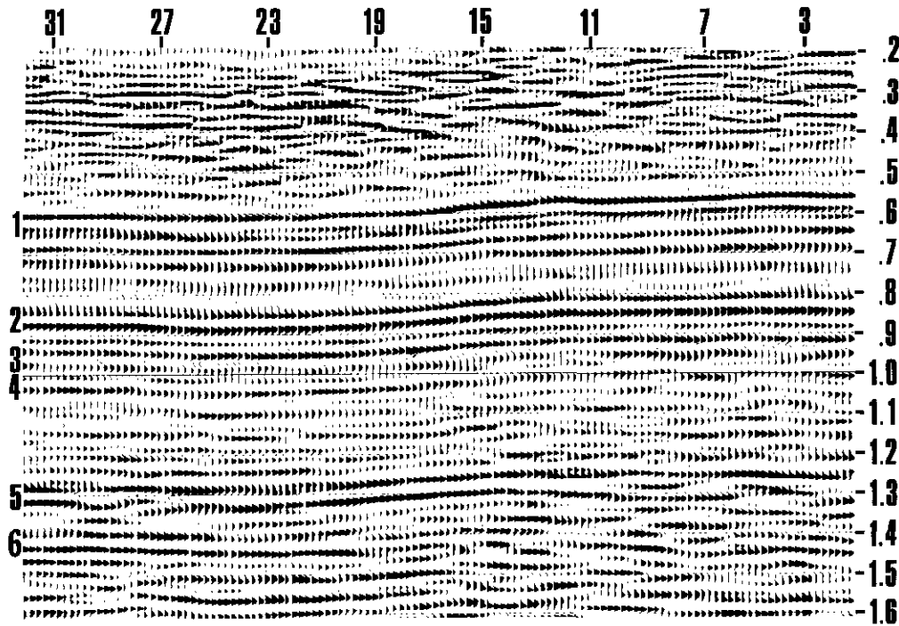
Fig. 5. Section in Figure 4 after two-dimensional (125 hz* 8 traces) filter.
