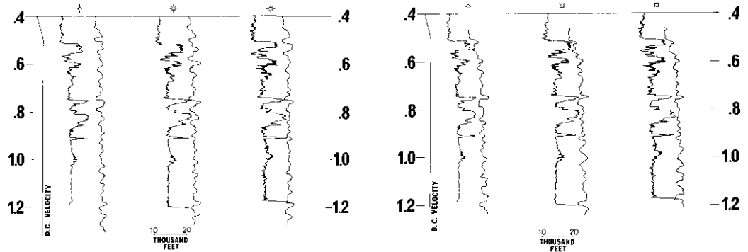
Fig. 10. Comparison of Sonic logs and inversion traces near three wells.
