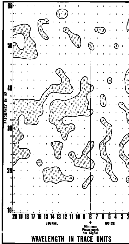
Fig. 3. Two-dimensional spectrum of a data set from Western Canada.
